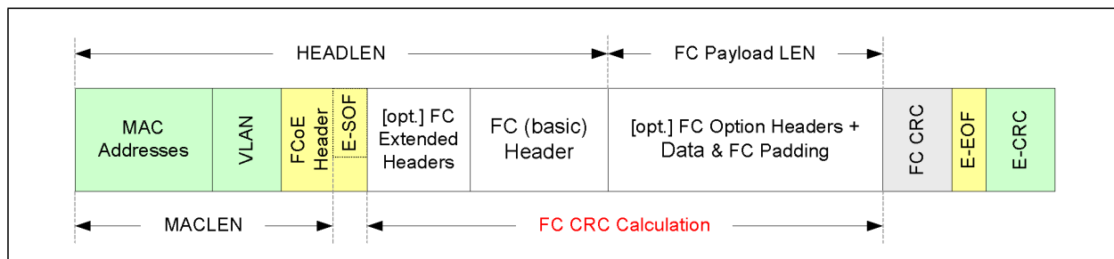
Figure 7.47 FCoE Frame and Relevant Transmit Descriptor Parameters
