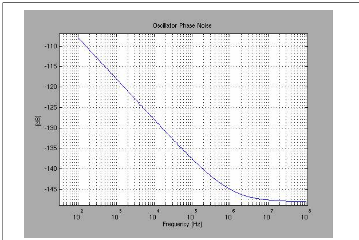
Figure 11.15 Maximum External Oscillator Phase Noise as a Function of Frequency (High-Speed Serial)
