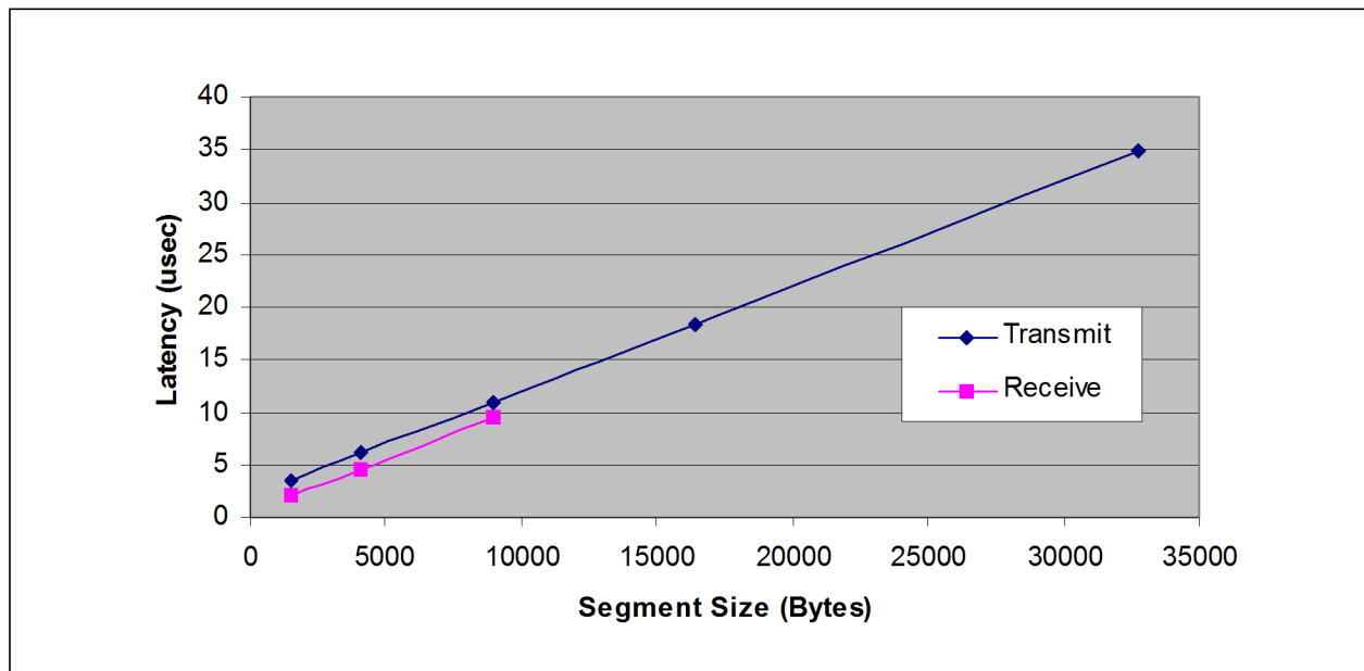
Figure 7.31 Latency Requirements
