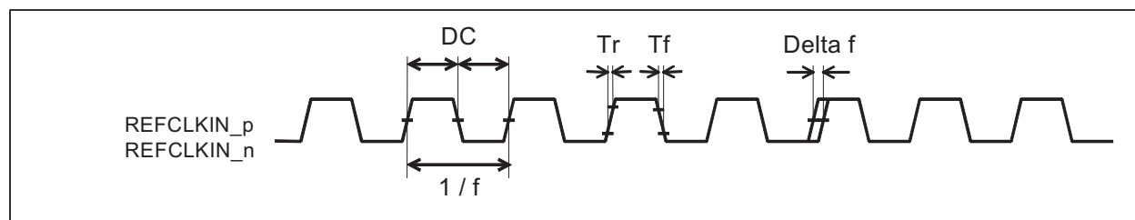
Figure 11.14 External Clock Reference Timing
