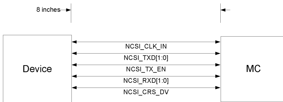
Figure 12.21 NC-SI Trace Length Requirement for Direct Connect
