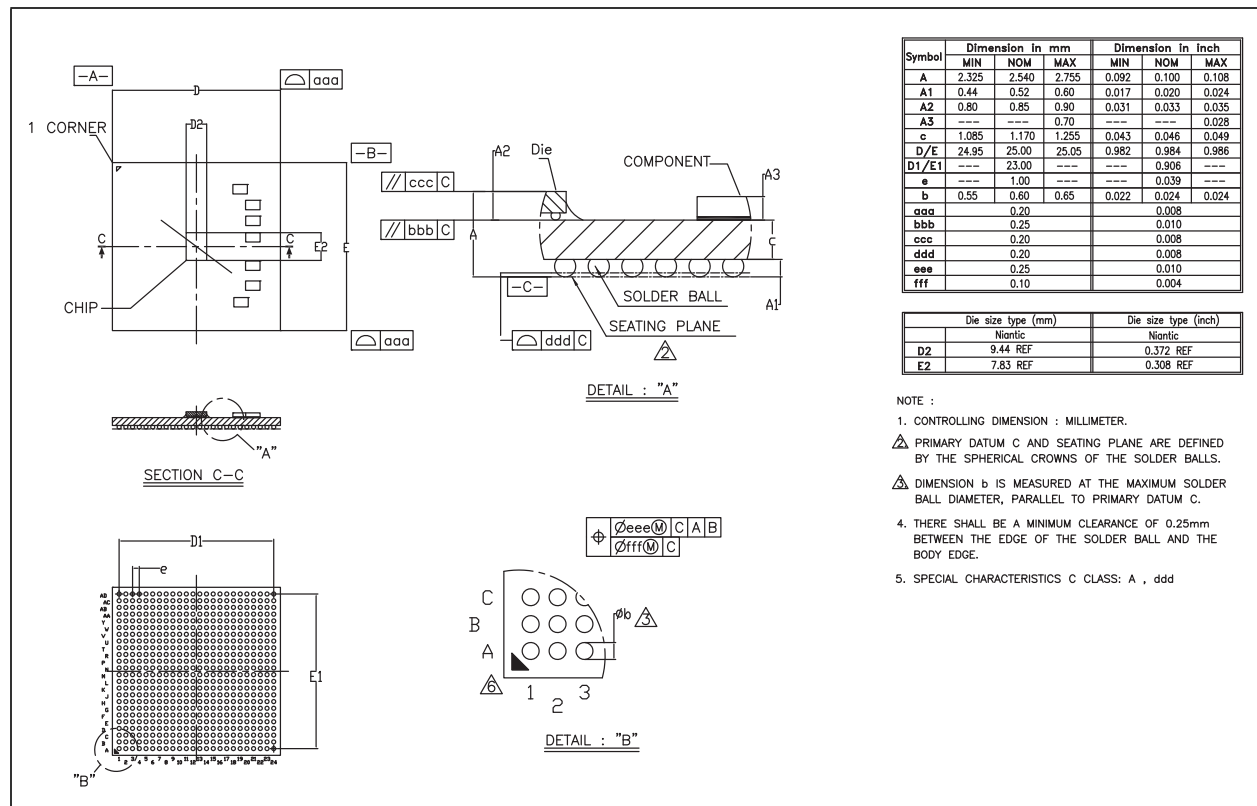
Figure 11.17 Mechanical Package
