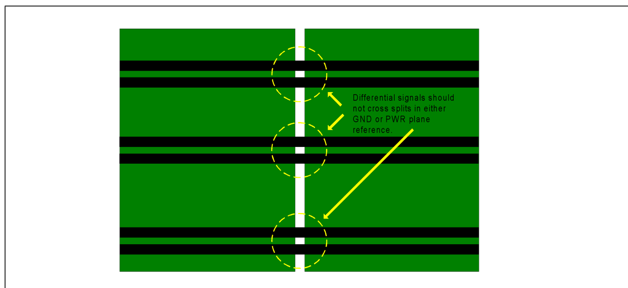
Figure 12.6 Do Not Cross Plane Splits
