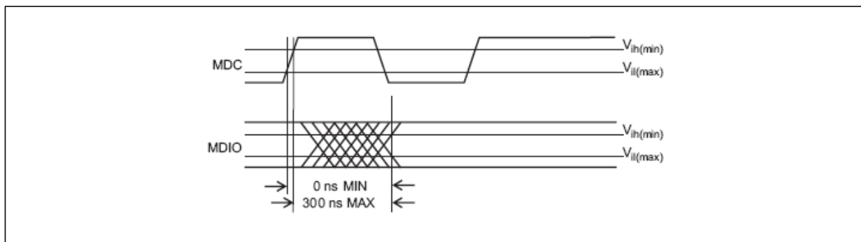
Figure 3.23 MDIO Timing Sourced by the PHY
