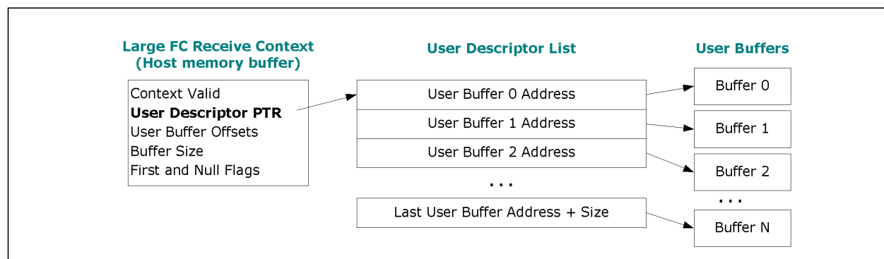
Figure 7.54 Large FC Receive Context Related to the User Buffers
