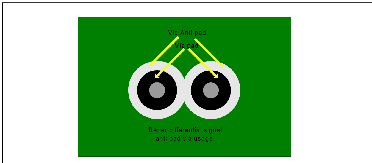
Figure 12.14 Better Differential Signals Via Anti-Pads
