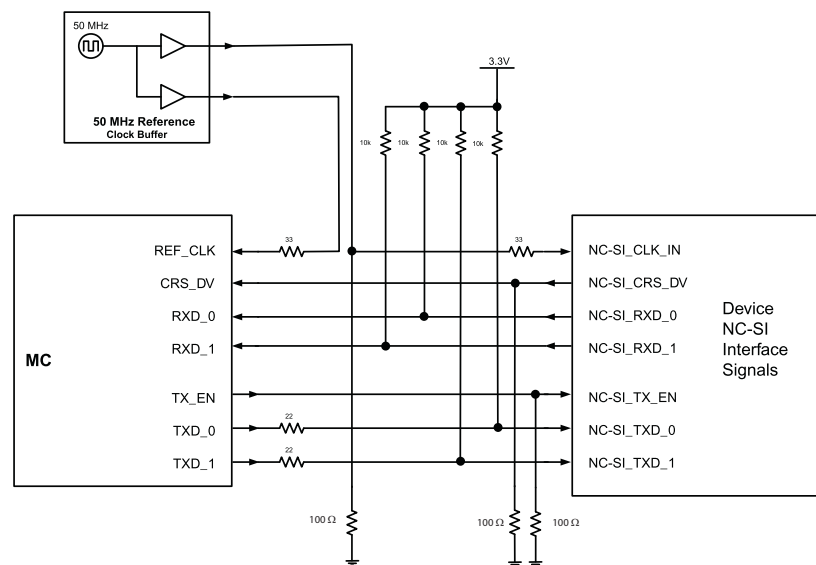
Figure 12.19 NC-SI Connection Schematic: Single-Drop Configuration
