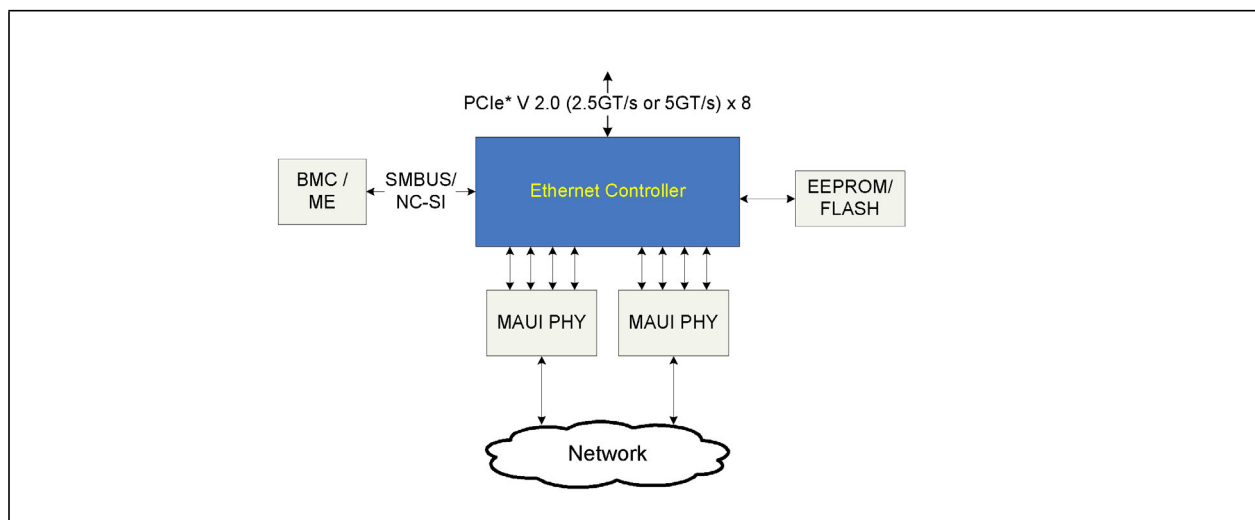
Figure 1.1 Typical Rack / Pedestal System Configuration
