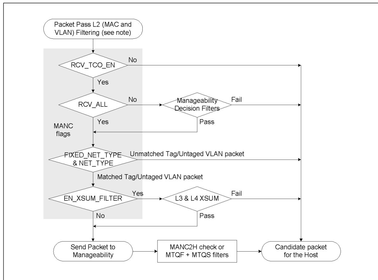
Figure 10.2 Flow Diagram
