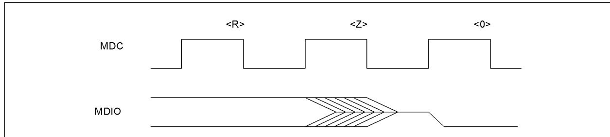
Figure 3.24 Behavior of MDIO During TA Field of a Read Transaction
