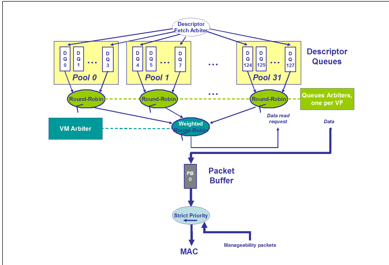
Figure 7.18 Transmit Architecture DCB-off/VT-on – 32 VFs
