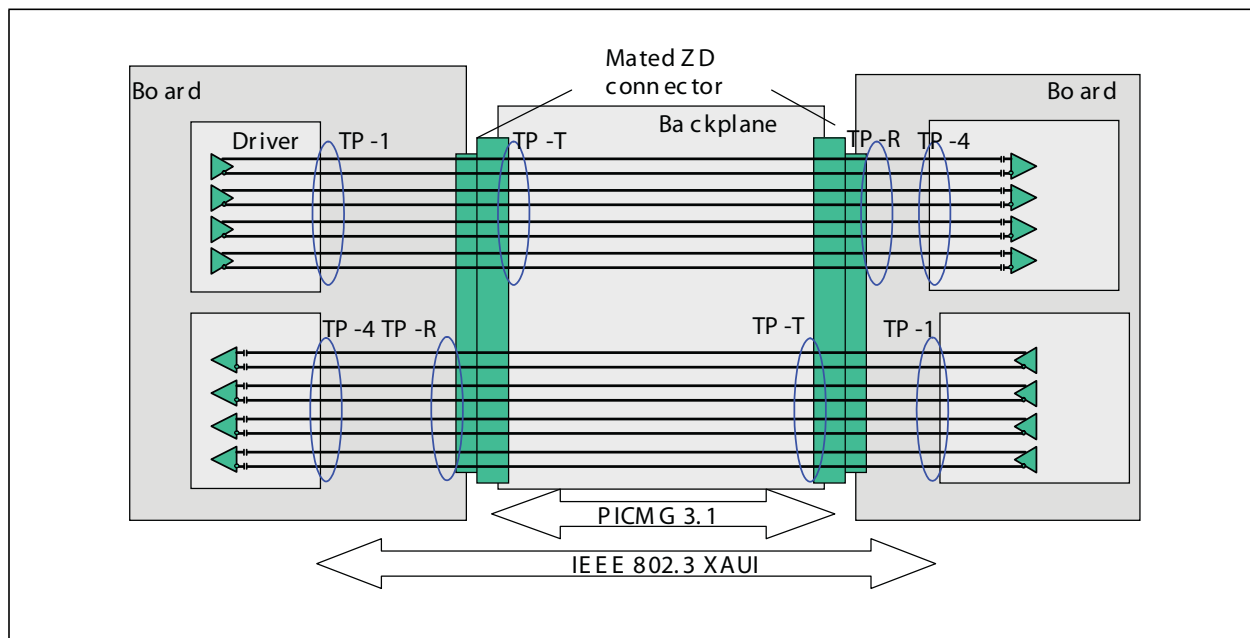
Figure 3.17 10GBASE-BX4 Electrical Environment
