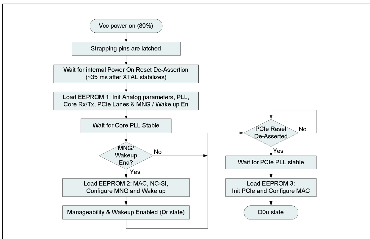
Figure 4.1 82599 Power-Up Sequence
