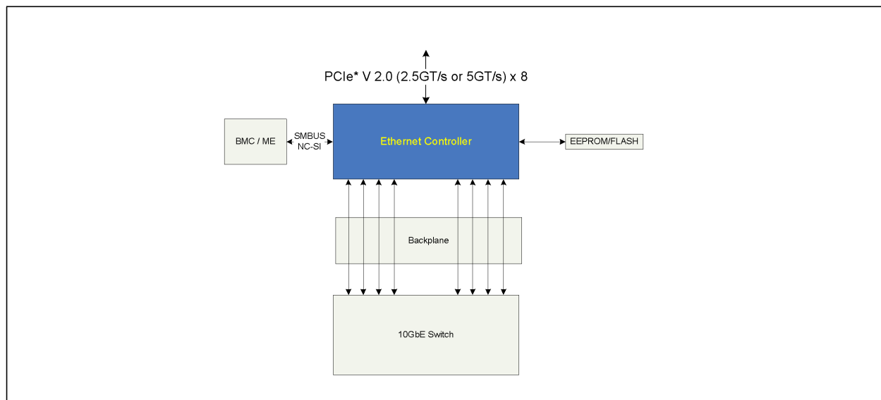
Figure 1.2 Typical Blade System Configuration
