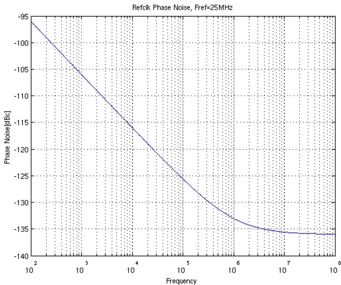
Figure 11.16 Refclk Phase Noise as a Function of Frequency (Non-High Speed Serial)
