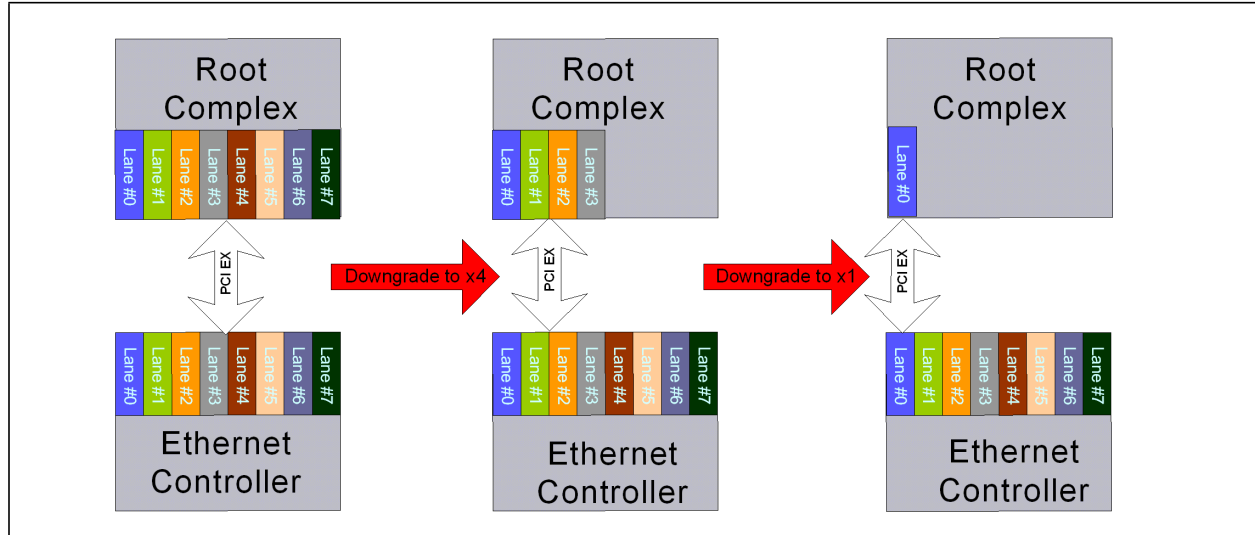
Figure 3.2 Lane Downshift in an x8 Configuration
