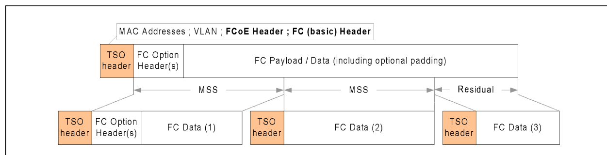
Figure 7.48 FCoE TSO Provided by the FCoE Driver
