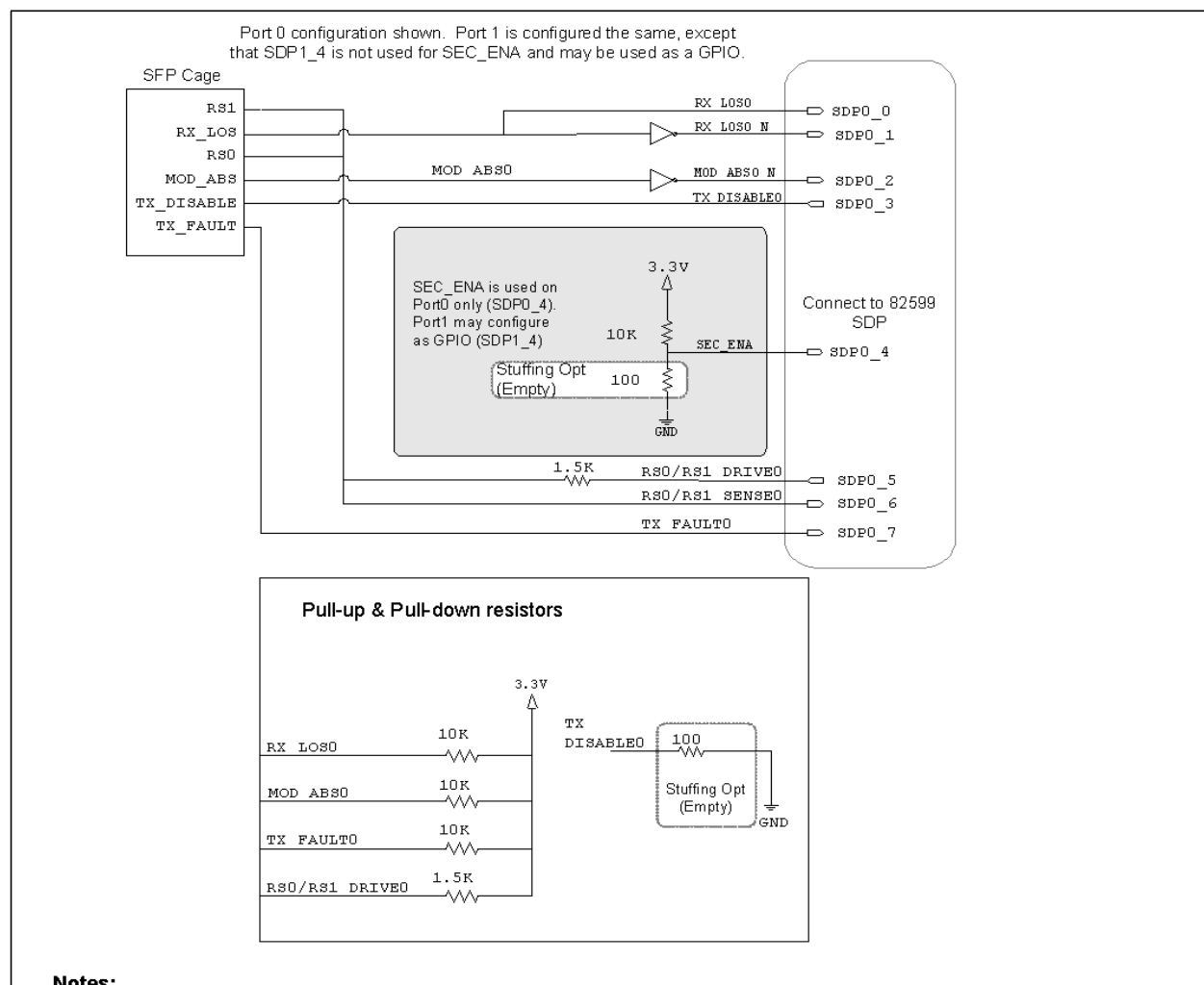
Figure 3.11 SDP Connections
