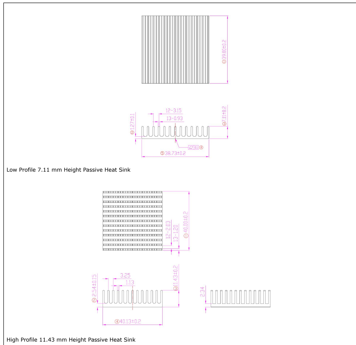
Figure 13.4 Extruded Heatsinks
