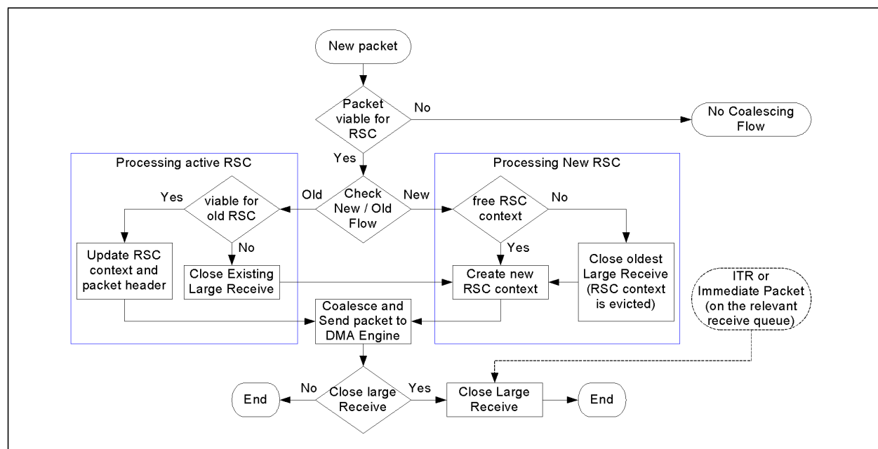
Figure 7.43 RSC Event Flow
