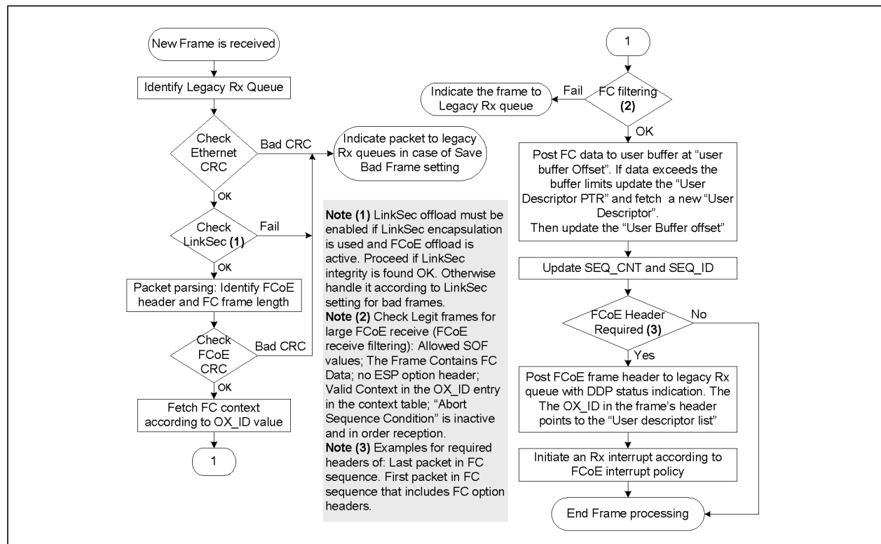
Figure 7.51 FCoE Large Receive Flow Diagram
