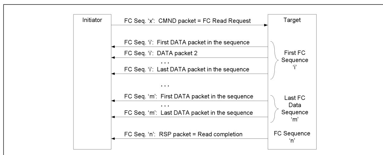
Figure 7.52 Example for FC Class 3 Read Exchange Flow
