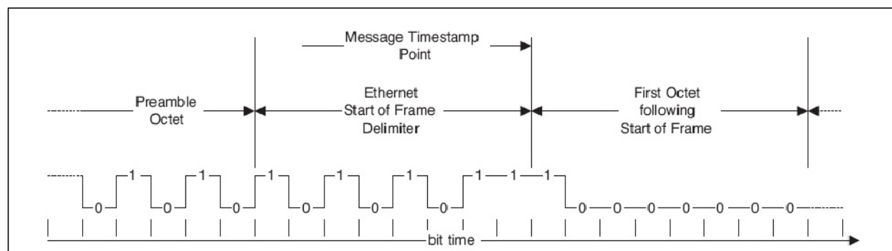
Figure 7.37 Time Stamp Point
