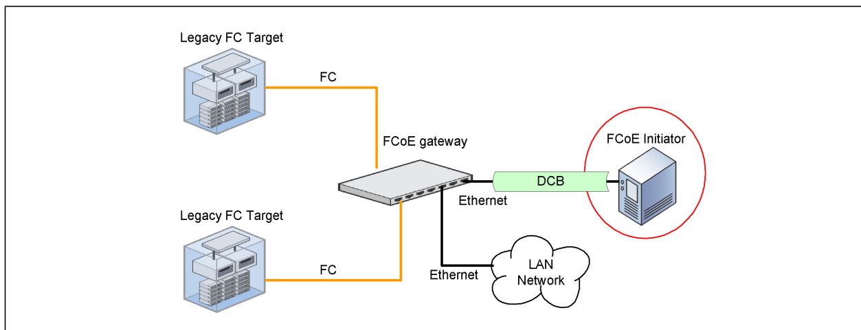
Figure 7.46 Connecting an FCoE Initiator to FC Targets
