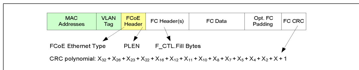
Figure 7.49 Relevant FCoE and FC Fields for CRC Receive Offload
