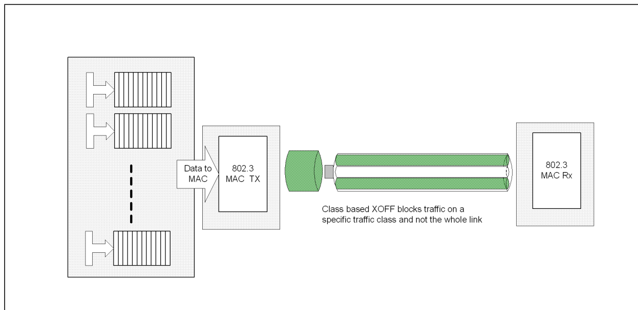
Figure 3.26 Priority Flow Control
