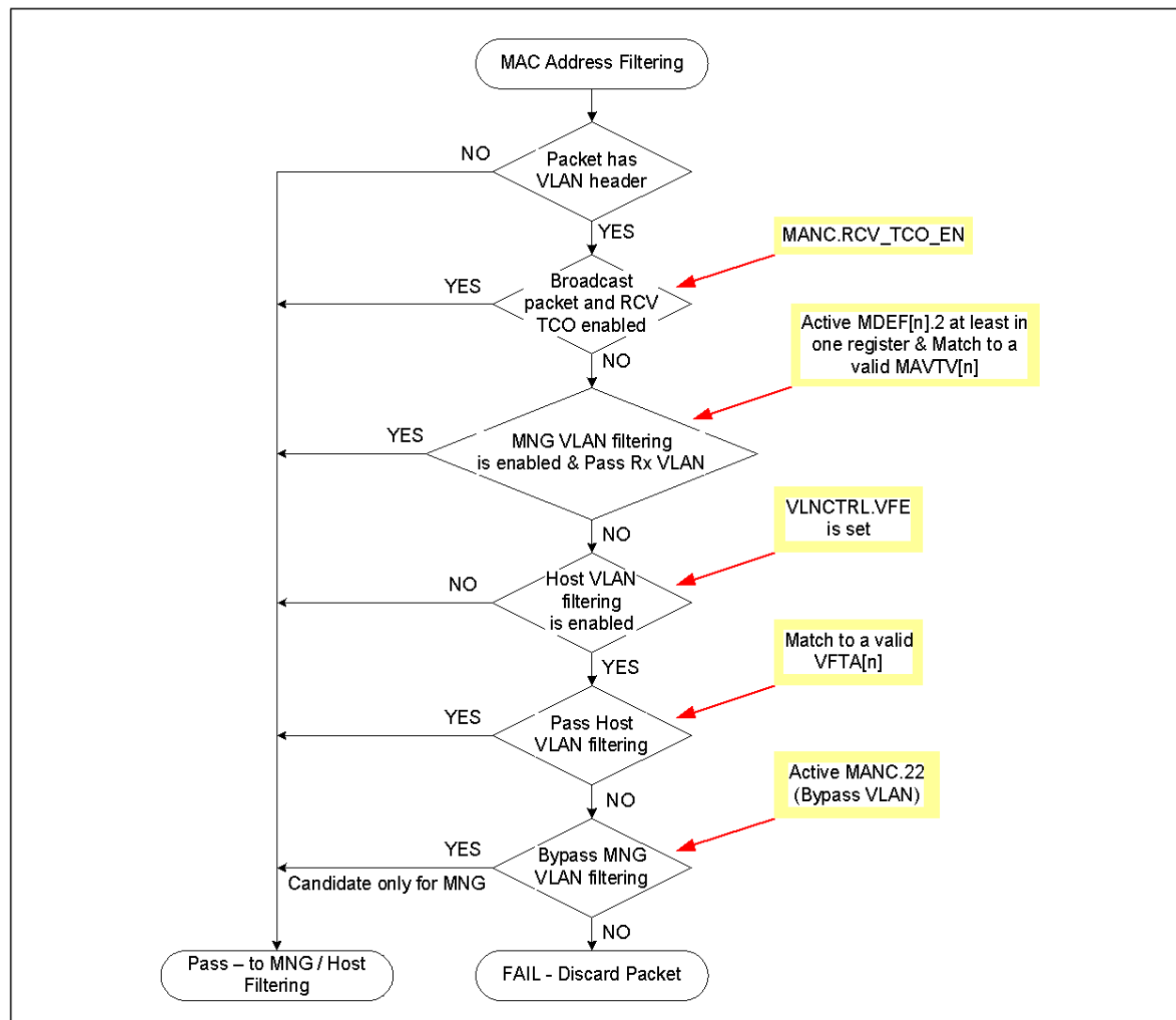
Figure 7.3 VLAN Filtering
