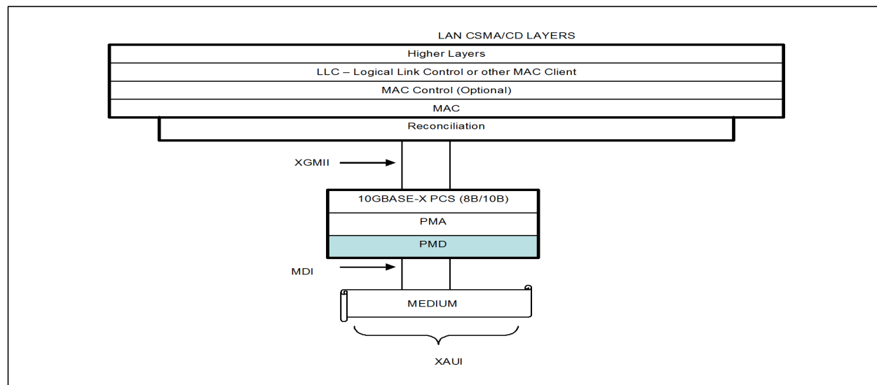
Figure 3.13 Architectural Positioning of XAUI
