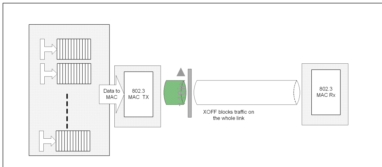
Figure 3.25 802.3X Link Flow Control (PAUSE)
