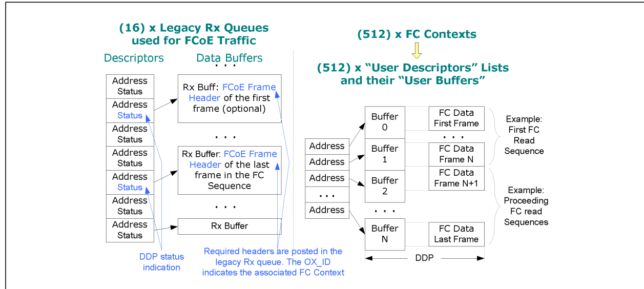
Figure 7.50 Large FC Reception to User Buffers and Legacy Rx Queue
