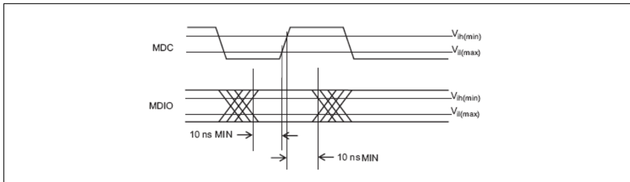
Figure 3.22 MDIO Timing Sourced by the MAC
