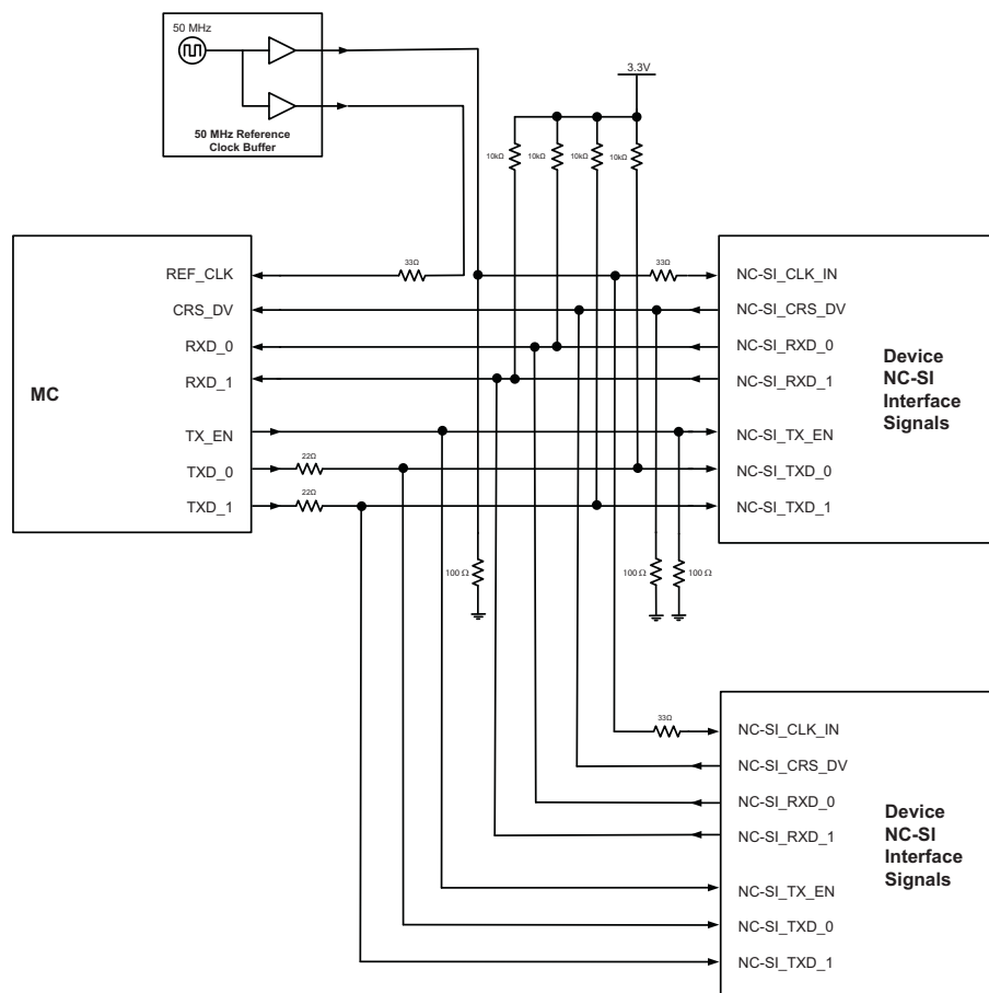
Figure 12.20 NC-SI Connection Schematic: Multi-Drop Configuration
