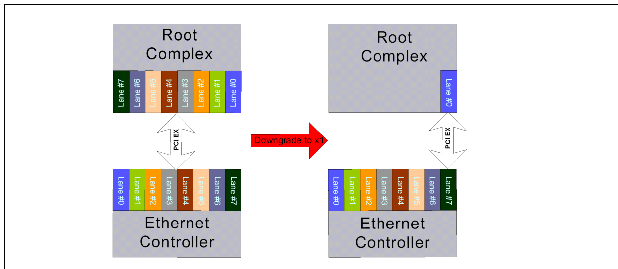
Figure 3.3 Lane Downshift in a Reversal x8 Configuration
