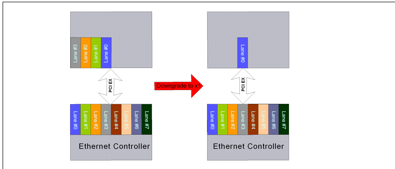
Figure 3.5 Lane Downshift in an x4 Reversal Configuration
