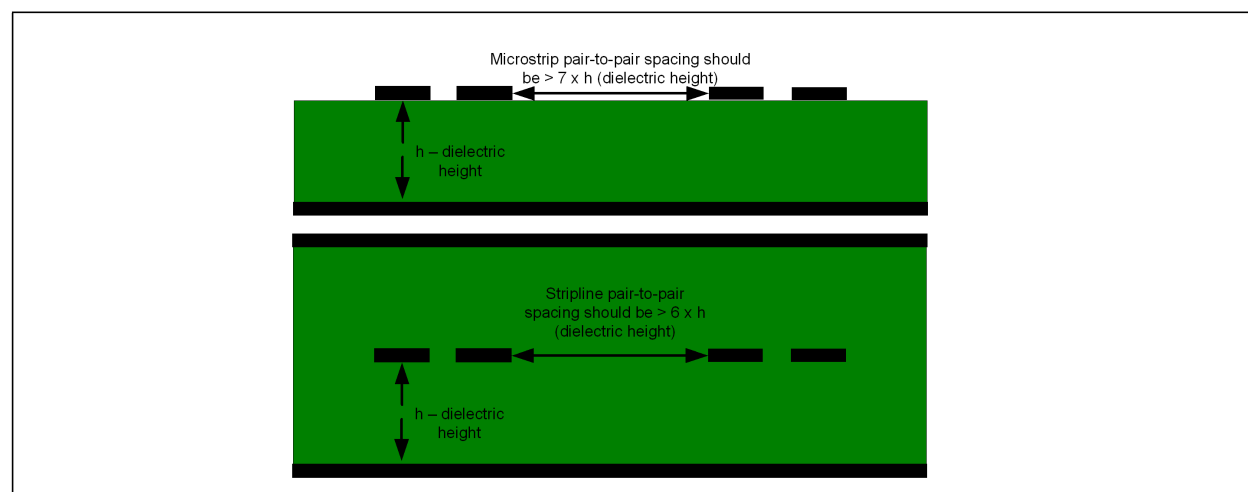
Figure 12.1 Differential Pair Spacing
