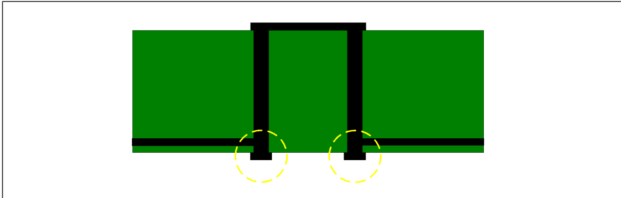
Figure 12.3 Correct Via Usage
