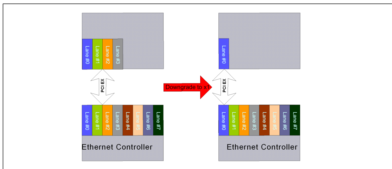
Figure 3.4 Lane Downshift in a x4 Configuration
