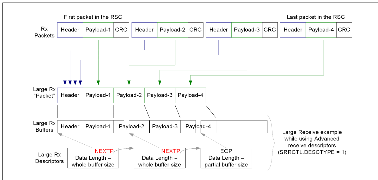
Figure 7.41 RSC Functionality (No Header Split)
