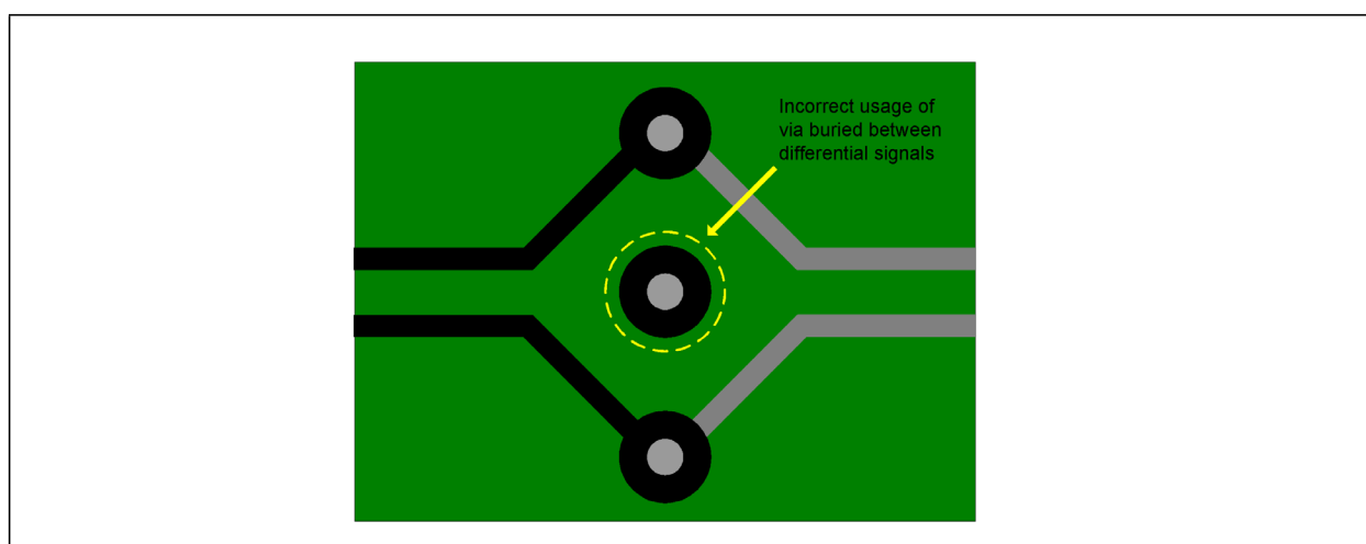
Figure 12.5 No Vias Between High-Speed Traces in the Same Differential Pair
