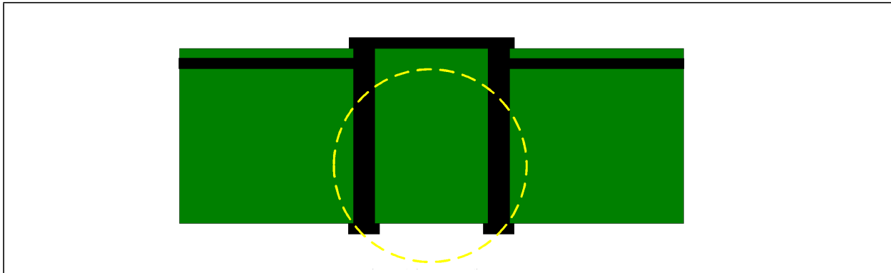
Figure 12.4 Incorrect Via Usage
