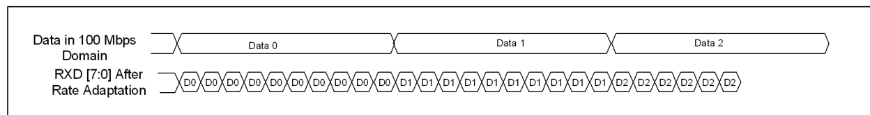
Figure 3.19 Data Sampling in 100 Mb/s Mode
